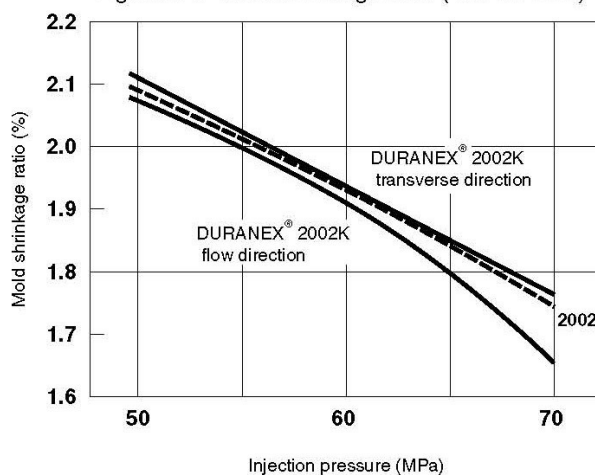
Figure 2-3 Mold shrinkage ratio (120×2 mmt)
